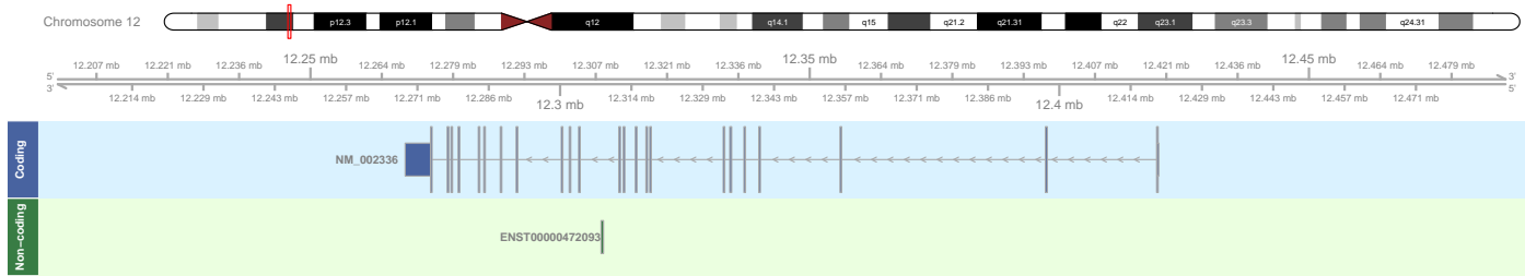
Figure 1. Genomic mapping showing the LncRNAs whose genes are located at or near the protein-coding gene LRP6.
