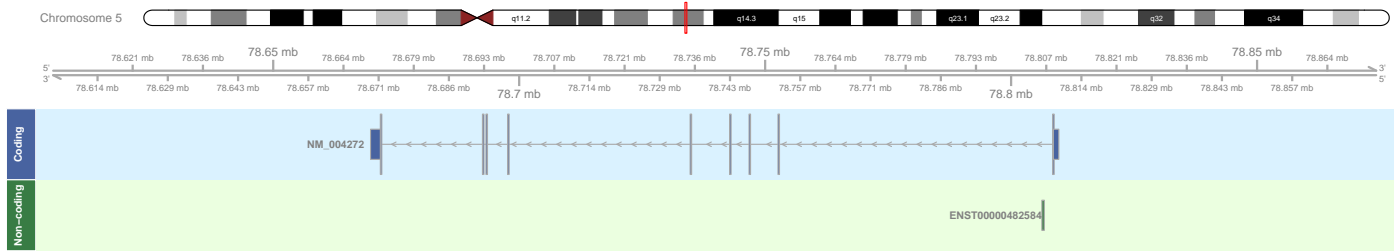
Figure 1. Genomic mapping showing the lncRNAs whose genes are located at or near the protein-coding gene HOMER1.
