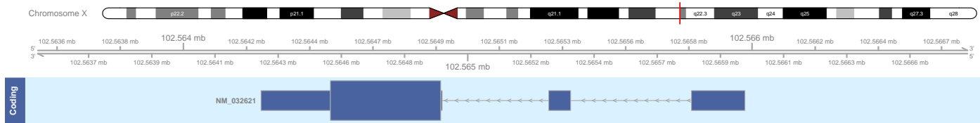
Figure 1. No nearby LncRNAs found for protein-coding gene BEX2.
